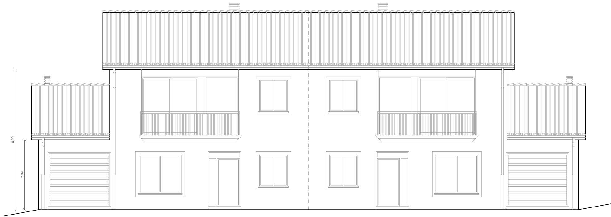
ALZADO PRINCIPAL
